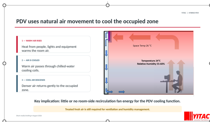
Figure 1. Warm air rises to the cooling coil; cooled, denser air descends gently into the occupied zone. Treated outdoor air is still required for ventilation and humidity control.
